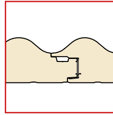
Concealed fixing
